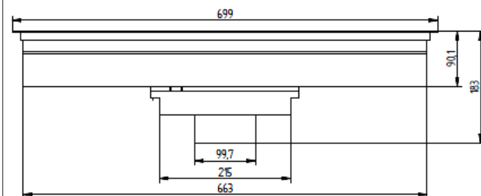
Product cut out dimensions 333 x 682mm
