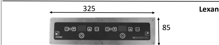
Control cut out dimensions 302 x 60mm
